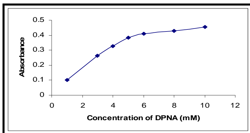
Fig.4: Effect of the concentration of DPNA (mM).
