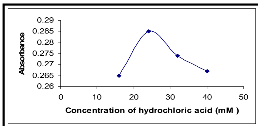
Fig.3: Effect of the concentration of HCL (mM).
