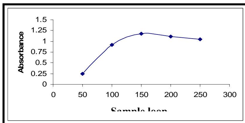
Fig.8: Effect of sample loop ( \mu l).
