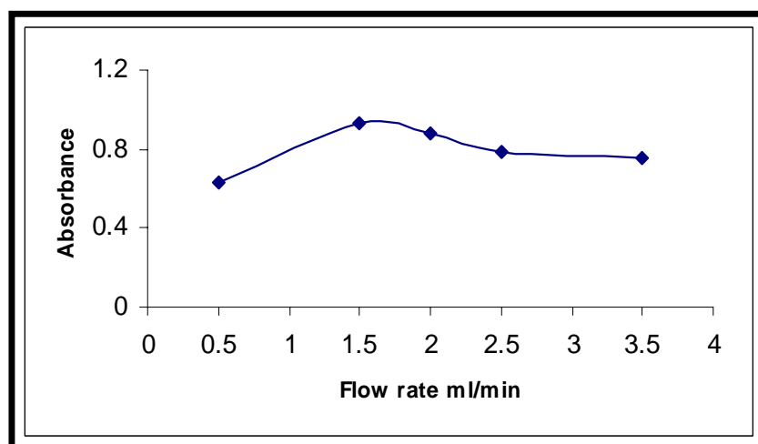
Fig.6: Effect of total flow rate (ml min -1 ).
